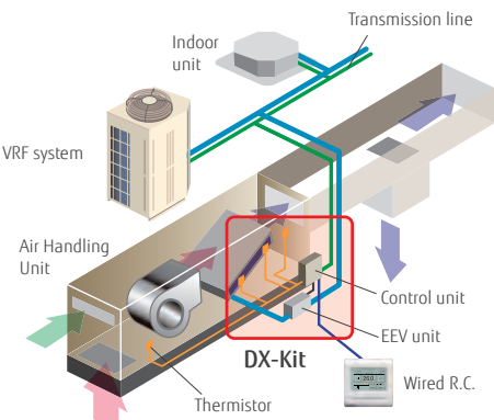
Arrangement as part of a VRF system
