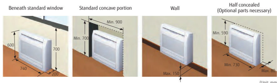
* Concaved position installation with concealment is prohibited. (Unit: mm)
